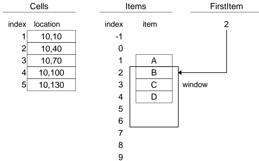
Figure E-6 - Presentation of few elements when WrapAround is False
