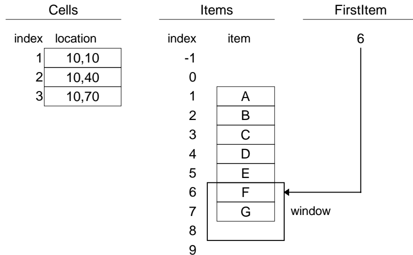
Figure E-4 - Presentation when WrapAround is False
