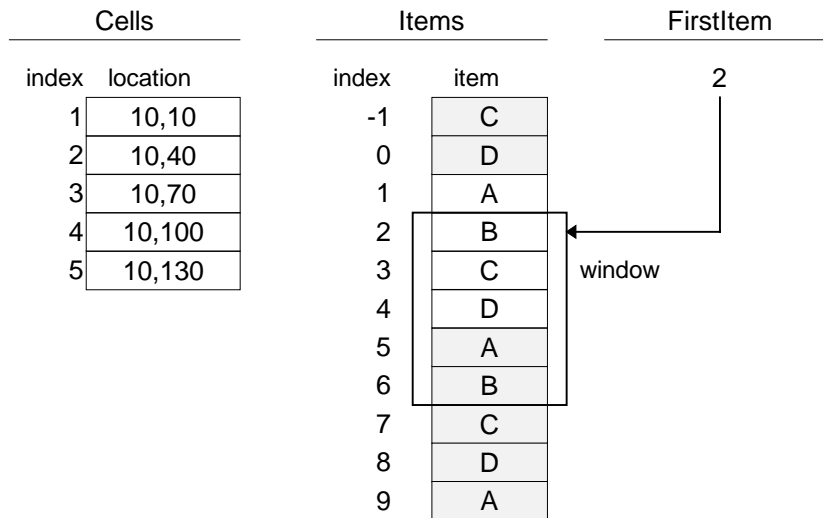
Figure E-7 - Presentation of few elements when WrapAround is True
