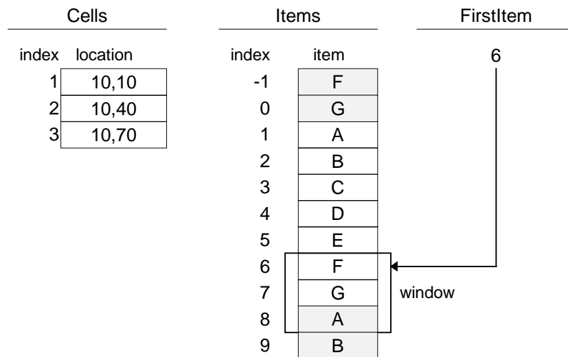
Figure E-5 - Presentation when WrapAround is True
