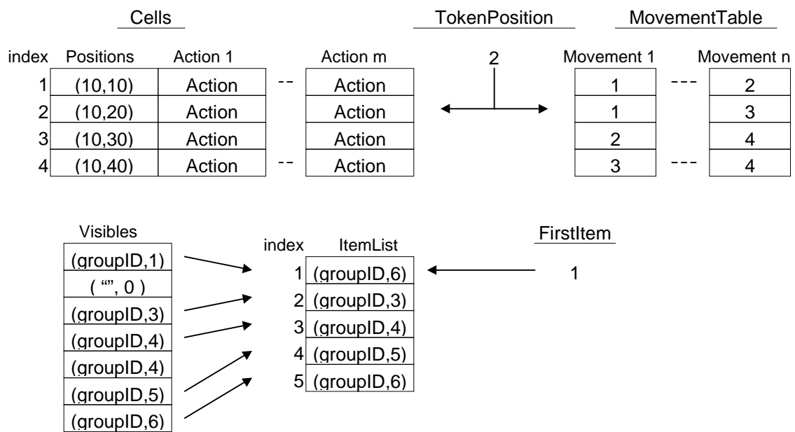
Figure E-3 – Preparation of ListGroup data structures
