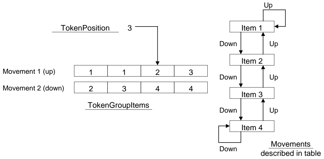
Figure E-1 – The MovementTable in TokenManager
