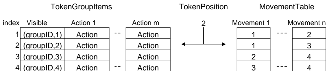
Figure E-2 – Data structures in TokenGroup
