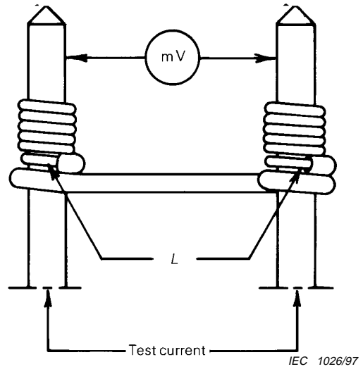
Figure 8b – Modified wrapped connections
