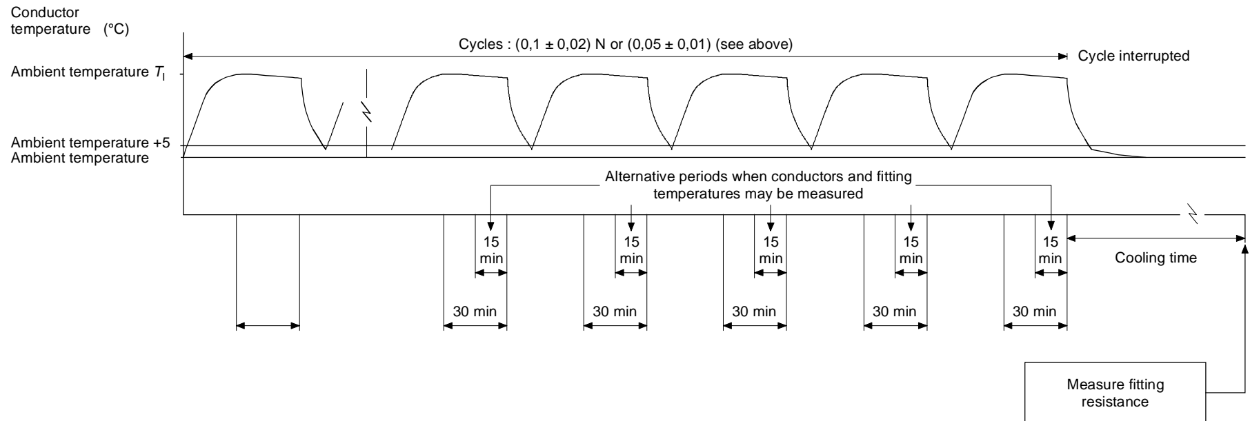
Figure D.2 - Detail of 0,1 N or 0,05 N cycle sequence
